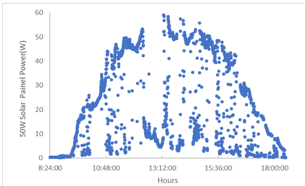
Fig. 7. PV power curve obtained during a blue-sky day after decreasing optimal voltage update limit.
