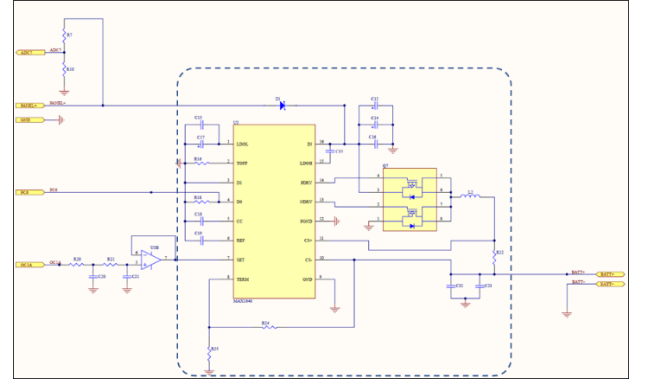
Fig. 3. Charger circuit for testing and tuning the MPPT algorithm.
