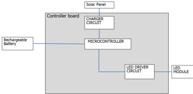
Fig. 2. Block diagram of the solar street light controller board.
