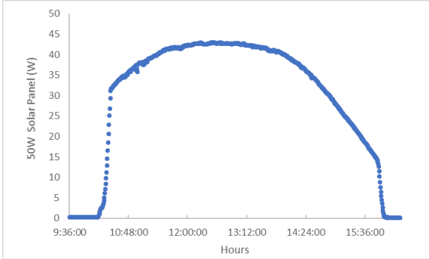
Fig. 5. Power measured of a 50W solar panel during a blue-sky day, using a 6.5 \Omega power resistor.
