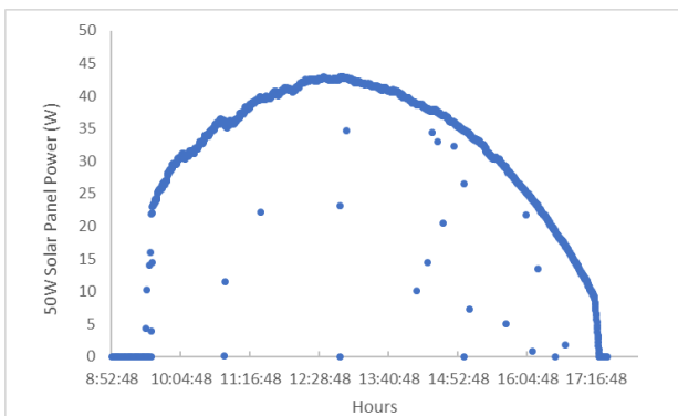
Fig. 8 - PV power curve obtained during a blue-sky day with the adjustment of the optimal voltage update limit.
