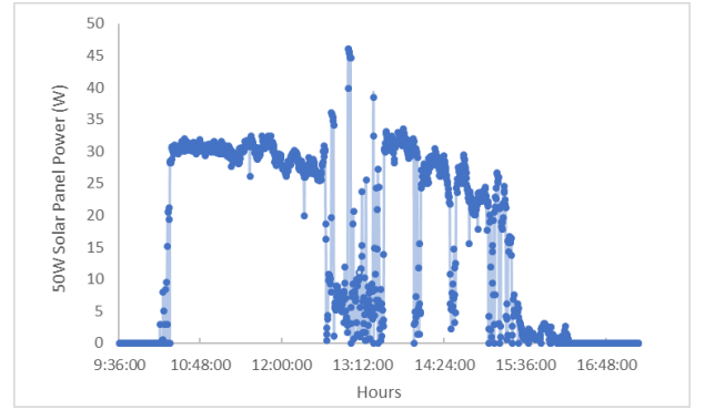
Fig. 6. PV power curve obtained during a blue-sky day after K_p was adjusted.
