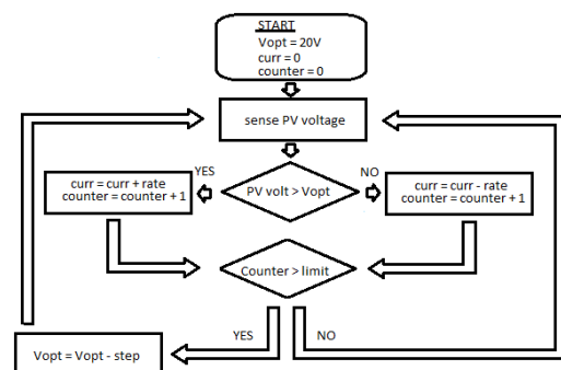
Fig. 1. Flow chart of the proposed MPPT algorithm.
